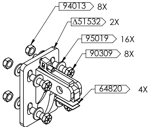
DETAIL D SCALE 1 : 6
