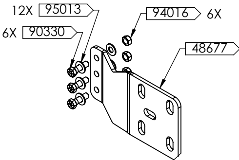
DETAIL C SCALE 1 : 6
