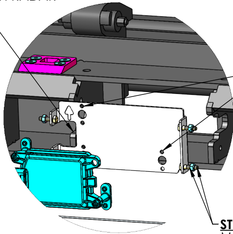
DETAIL E SCALE 1 : 6
