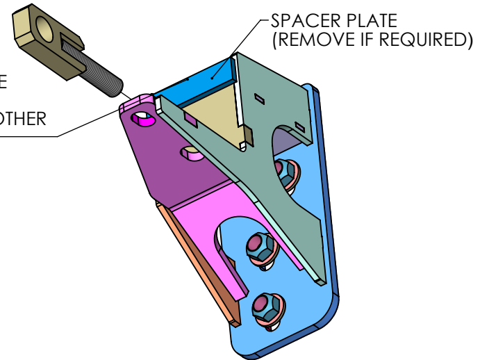
MOUNTING BRACKET ASSEMBLY
